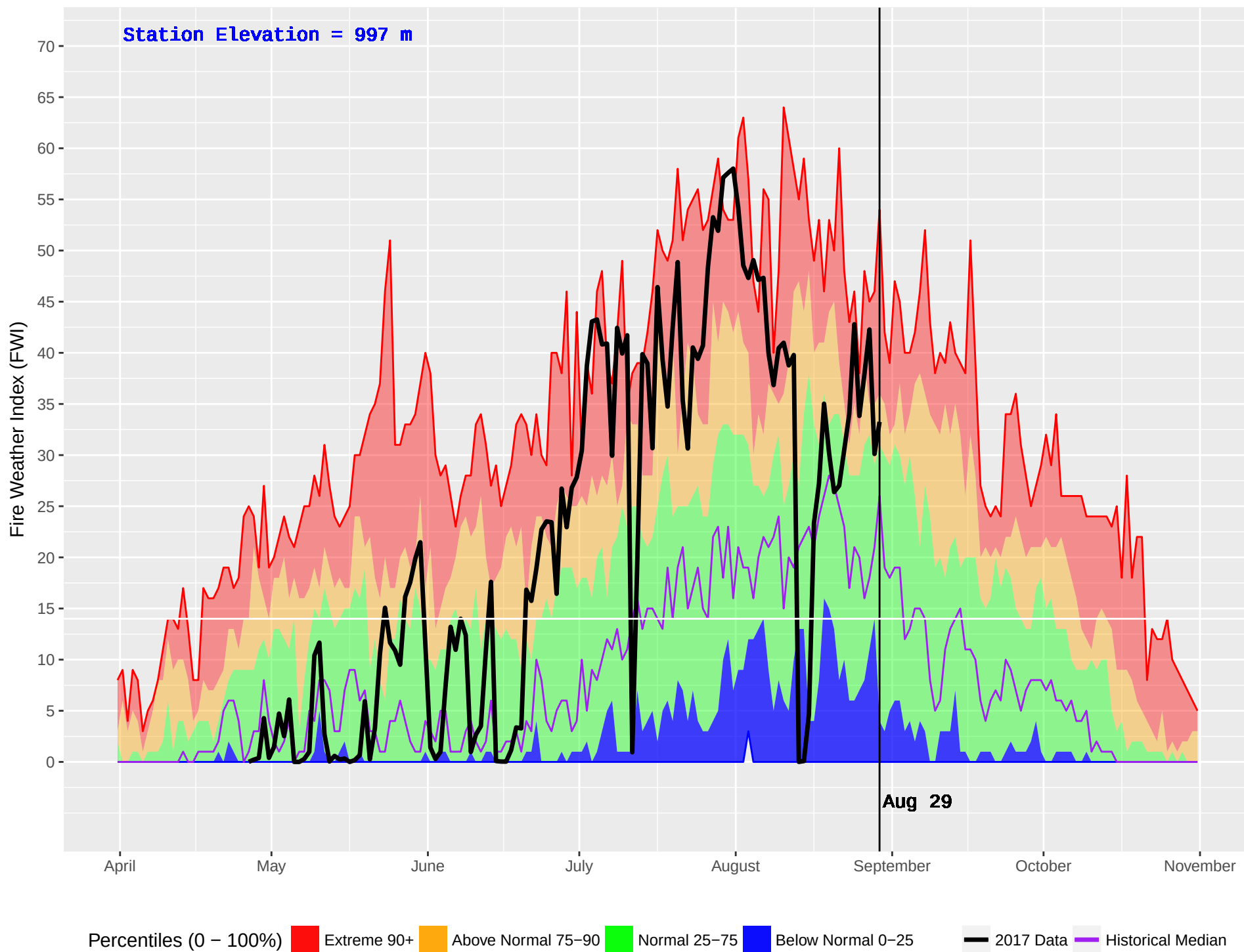
SMALLWOOD (404) : Historical (1991–2016) and Current (2017) Noon Fire Weather Index (FWI)
