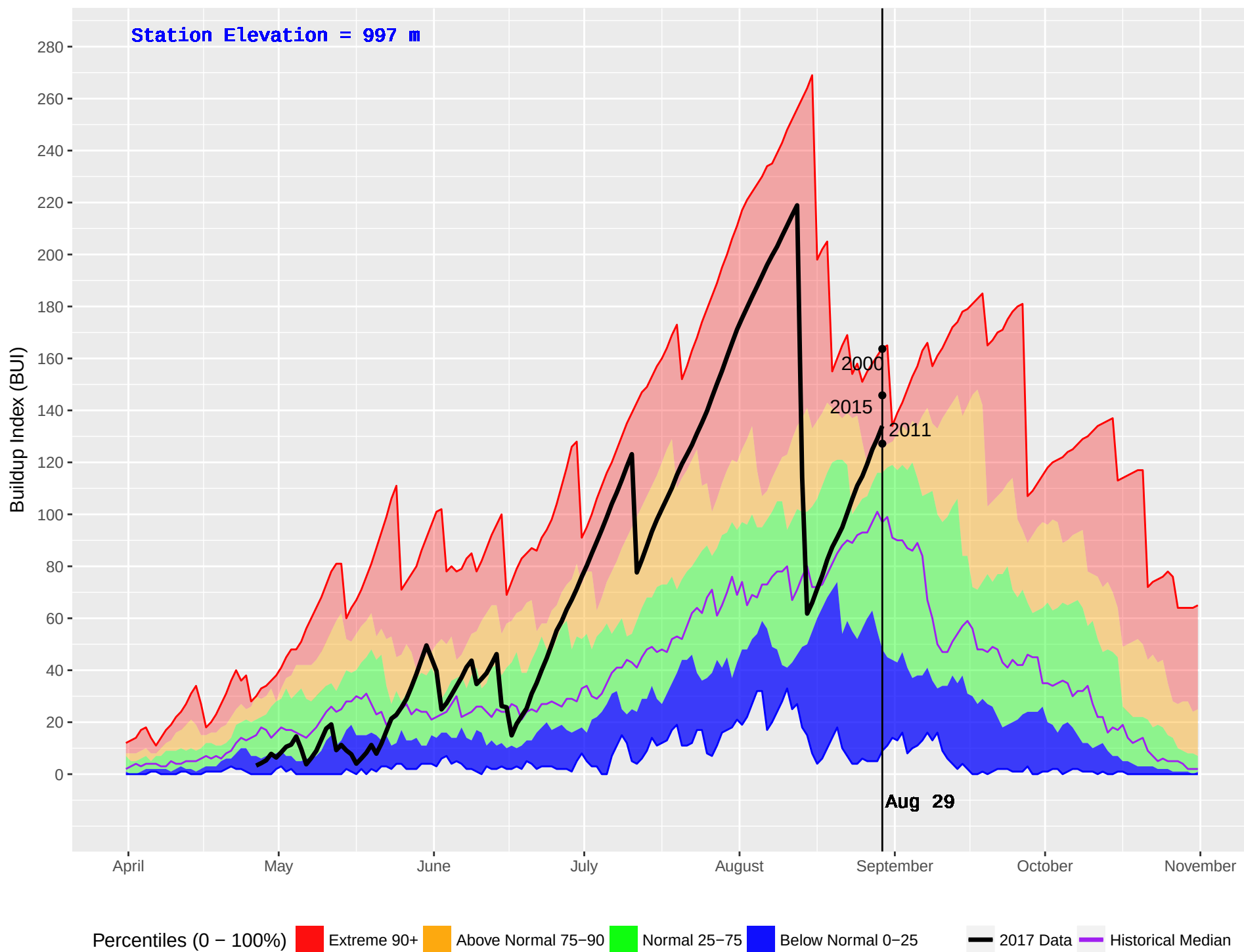
SMALLWOOD (404) : Historical (1991–2016) and Current (2017) Noon Buildup Index (BUI)
